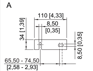
Wall mounting bracket fitted in mounting rail
